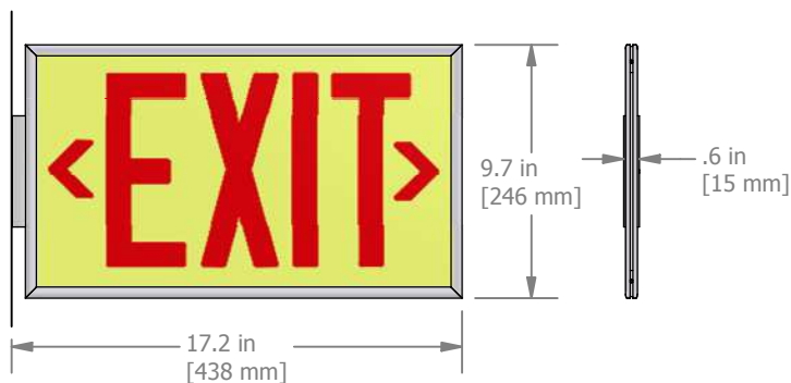
EDGE MOUNTED
