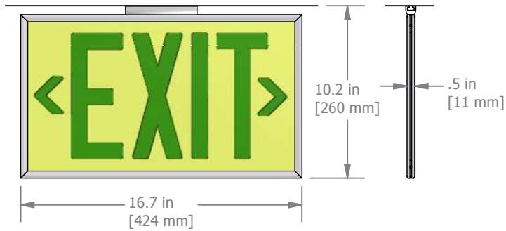
CEILING MOUNTED
